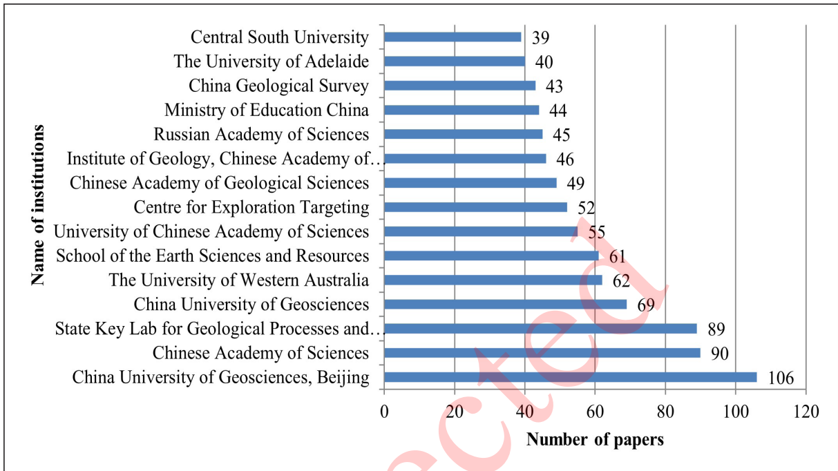
Figure 8- List of top 15 published institutions on gold deposits and mineralization.
