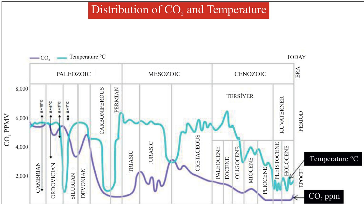
Figure 36- Diagram showing that during the geologic past CO 2 level was much higher than the present level of 420 ppm. Note that there is no correlation between Temperature and CO 2 trends (Epstein, 2022). Portfolio/Penguin (Berner, 1991, 2004; Scotese et al., 2021). Additional labels by G. Shanmugam.
